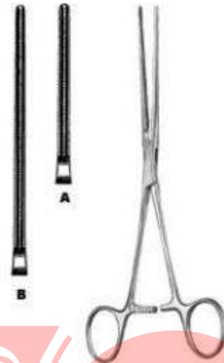
Bainbridge BI-9-168-15 Multipurpose Vascular Clamp 15cm,
